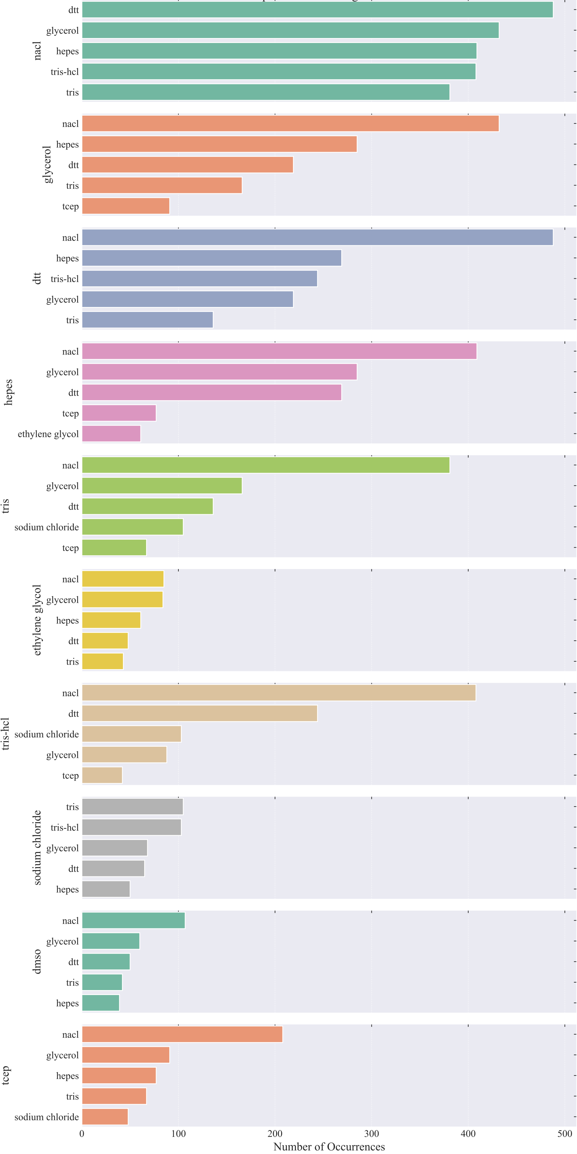
Most Common partners for missing words
